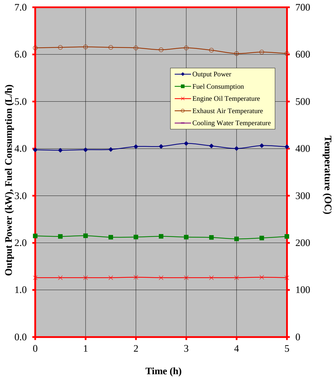
Figure 4. Performance characteristic curves during the continuous running test of the HONDA GX270H QHPI gasoline engine
