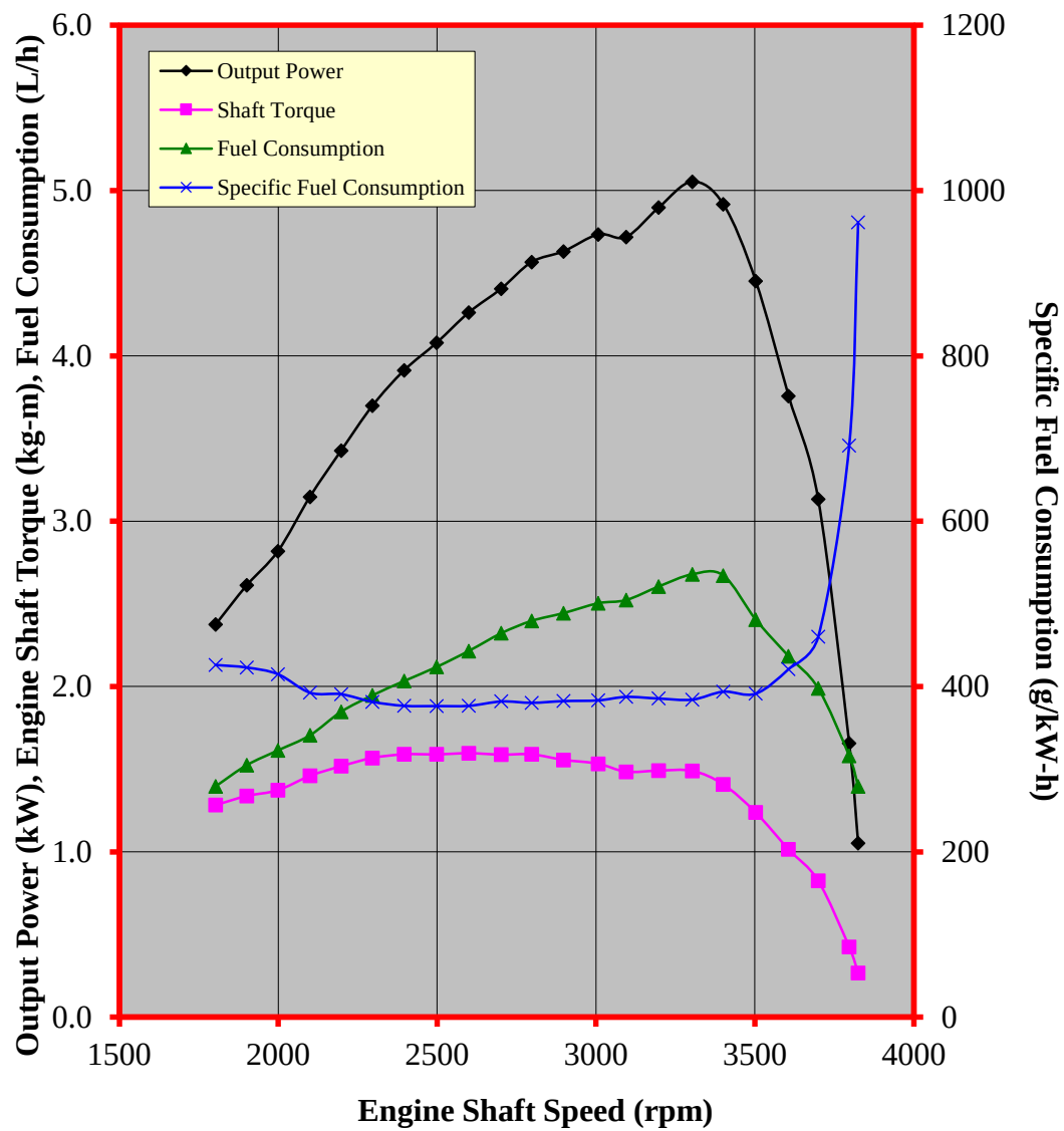
Figure 3. Performance characteristic curves of the HONDA GX270H QHPI gasoline engine
